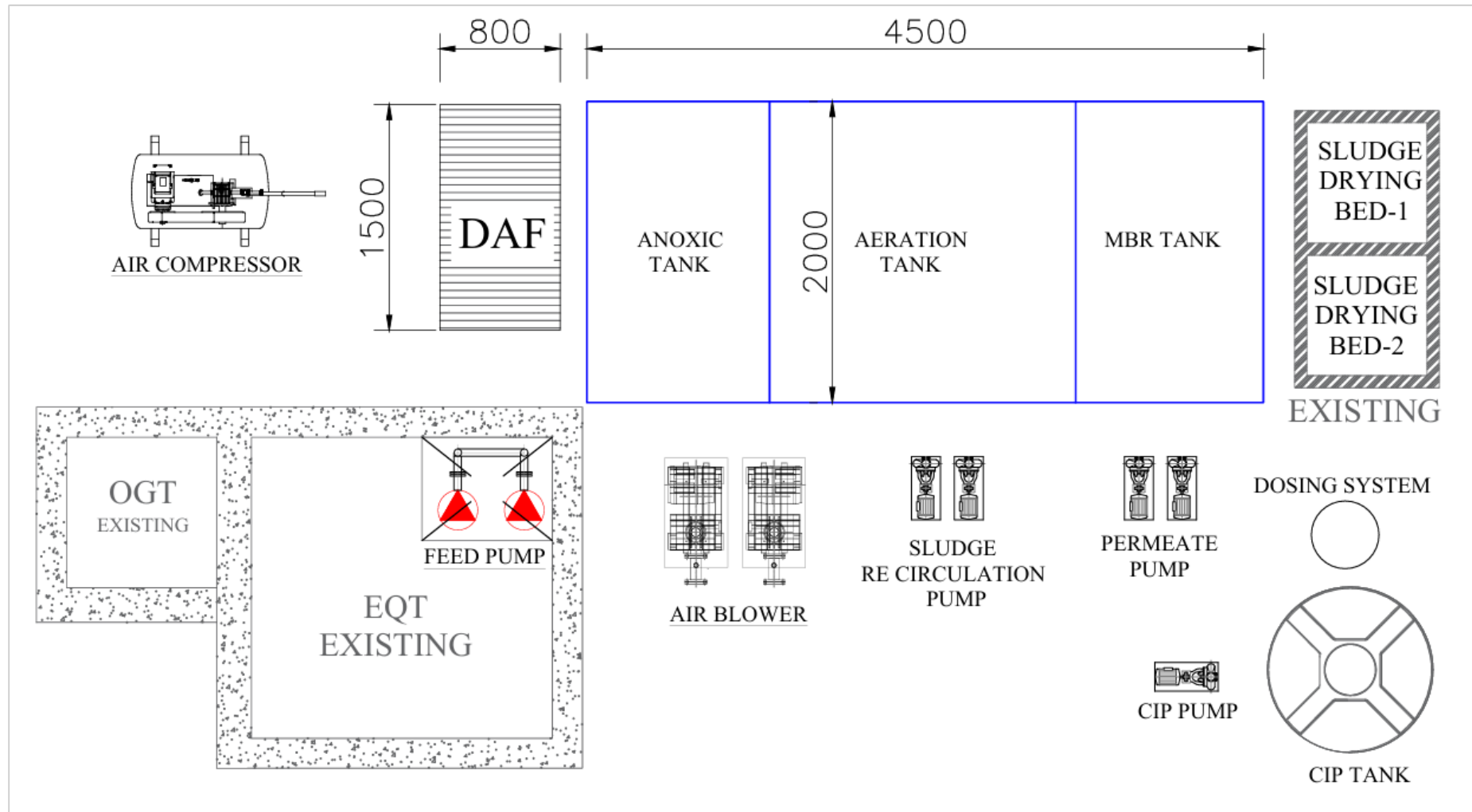
GA LAYOUT PLAN – EFFLUENT TREATMENT PLANT
